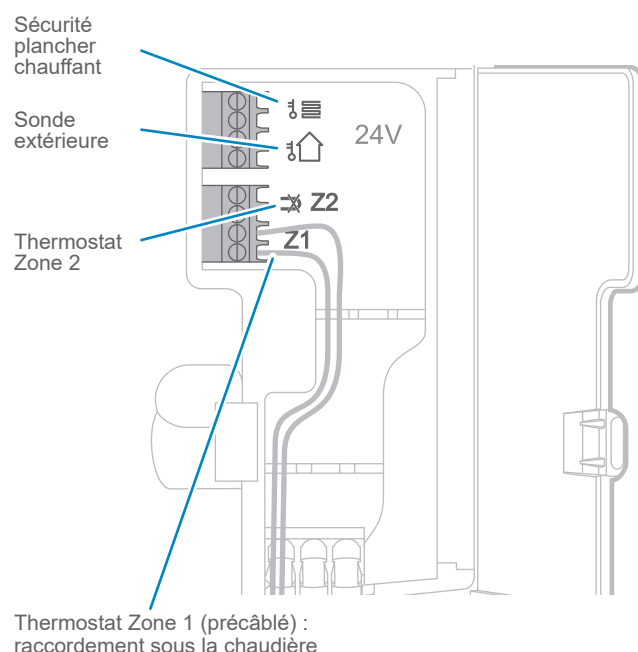
fig. 18 - Borniers TBTS
